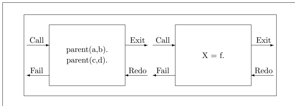
Figure 5.1: The Byrd Box Model Illustrated
