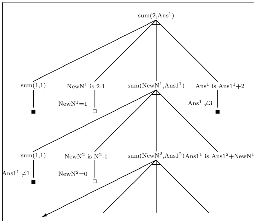
Figure 9.3: Resatisfying the Goal \text{sum}(2, \text{Ans})
