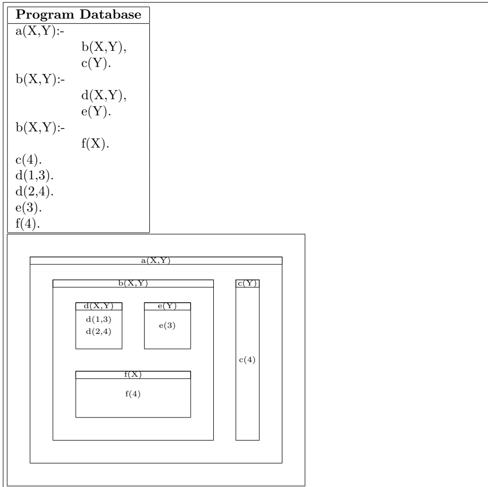
Figure 5.3: Program Example with Byrd Box Representation
